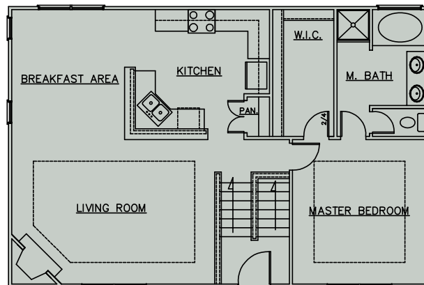
SECOND FLOOR - PLAN B
