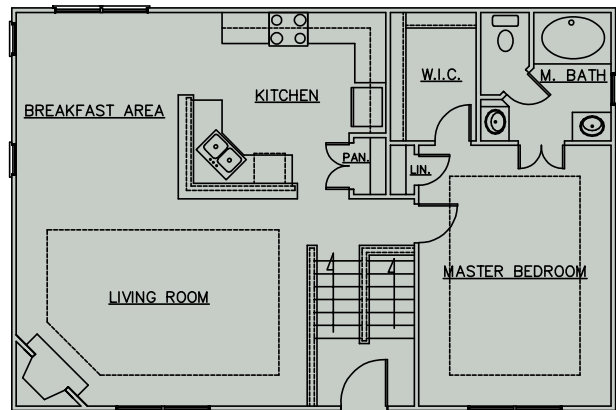
SECOND FLOOR - PLAN A
