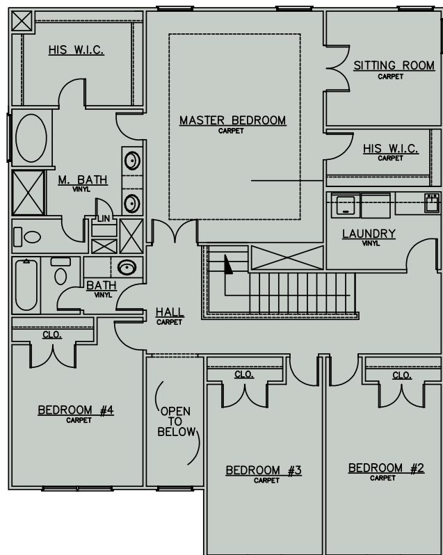
SECOND FLOOR
